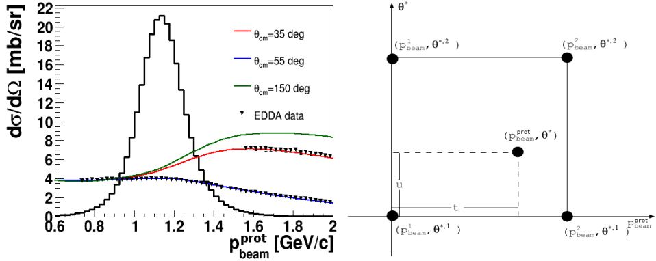
Fig. 4. Left: Differential cross sections for proton–proton elastic scattering as a function of the beam momentum for a three values of the scattering angle \theta^* in the CM frame. Black points show EDDA Collaboration data [39], while lines denote SAID calculations [38]. Distribution of the effective beam momentum for quasi-free pp \rightarrow pp reaction calculated for the deuteron beam momentum range p_{\text{beam}} \in (2.127, 2.422) GeV/ c is also presented in the figure. Right: Bilinear interpolation of the differential cross section \frac{d\sigma}{d\Omega}(p_{\text{beam}}^{\text{prot}}, \theta^*) . The figure is adapted from [36].
