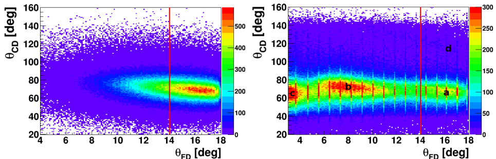
Fig. 6. Correlations between the polar angles \theta_{\text{FD}} and \theta_{\text{CD}} for the WMC Simulations of dd \rightarrow ppn_{\text{sp}}n_{\text{sp}} reaction (left panel) and obtained in experiment (right panel). Applied cut is marked with vertical/red line. The indicated area correspond to the: (a) dd \rightarrow ppn_{\text{sp}}n_{\text{sp}} , (b) dd \rightarrow d_b p_t n_{\text{sp}} and dd \rightarrow ppn_{\text{sp}}n_{\text{sp}} , (c) dd \rightarrow pp_{\text{sp}}nn_{\text{sp}} , (d) dd \rightarrow p_b d_t n_{\text{sp}} .
