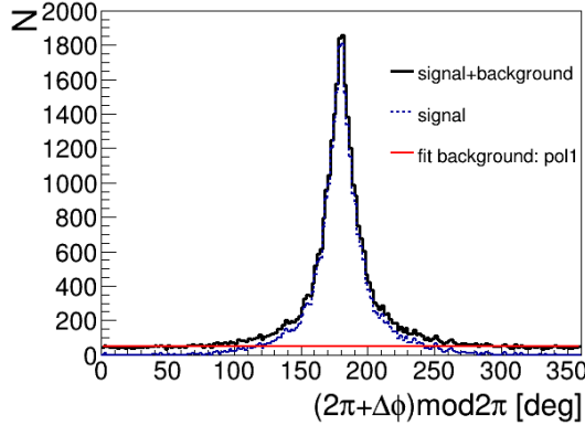
Fig. 7. Distributions of (2\pi + \Delta\phi)\text{mod}2\pi , where \Delta\phi = \phi_{\text{CD}} - \phi_{\text{FD}} is the difference of azimuthal angles in the Central Detector and Forward Detector. The example spectrum for one of the Q intervals (solid/black line) with marked fit function (horizontal/red line) and signal peak after background subtraction (dotted/blue line) is presented.
