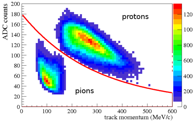
Fig. 1 dE/dx (in ADC counts) vs. momentum for the selected proton (up) and pion (down) tracks in the final selection. The proton selection functions is displayed in red
