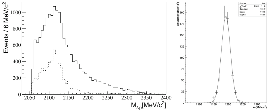
Fig. 3 Left: \Lambda p invariant mass for the inclusive \Lambda p selection (continuous line) and for events with an extra \pi^- detected (dashed line, arbitrary normalization). Right: m_{\Lambda\gamma_3} invariant mass distribution, together with a Gaussian fit
