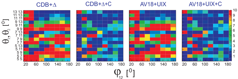
Fig. 1. Set \chi^2/\text{d.o.f.} values obtained for the differential cross sections and compared to various theoretical predictions. Cells of the map refer to individual configurations defined by the polar angles of two outgoing protons, \theta_1 , \theta_2 , and their relative azimuthal angle \phi_{12} .
